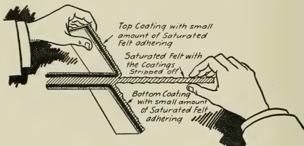
FIG. 203.—Method of Stripping the Coatings from the Saturated Felt.
